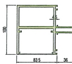
幕墙横梁•Y200-16 \delta=3.3 6.537 \frac{kg}{m}
