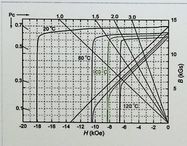
•50H Demagnetization Curve ( II - ⑤ )
