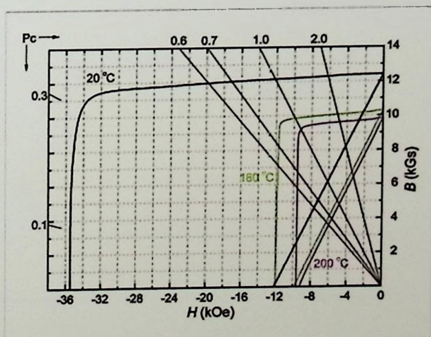
• 38AH Demagnetization Curves ( II - ① )
