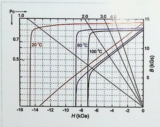
•45M Demagnetization Curve ( II - ⑧ )
