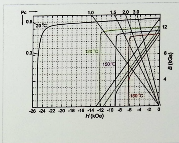
• 45UH Demagnetization Curve ( II - ③ )
