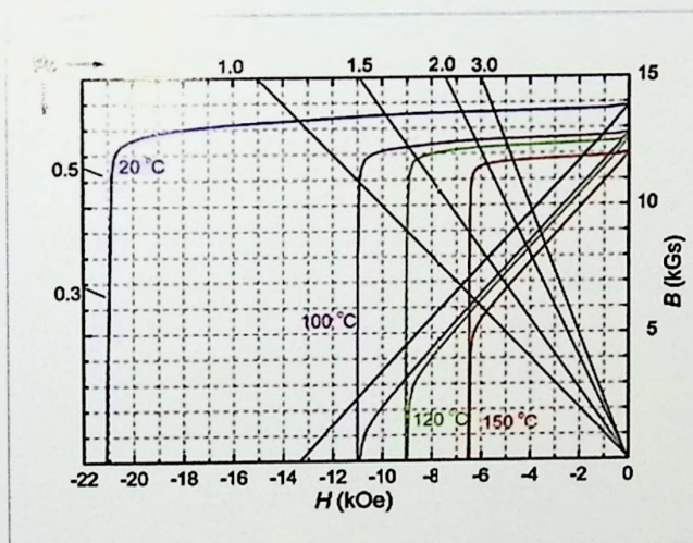
• 45SH Demagnetization Curve ( II - ④ )
