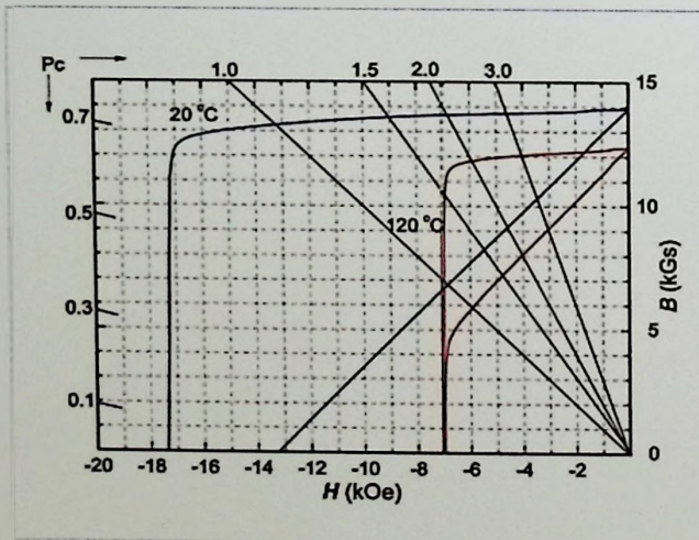
•Dy48H Demagnetization Curve ( II - ⑥ )
