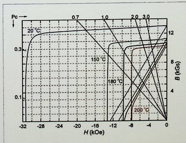
• 42EH Demagnetization Curves ( II - ② )
