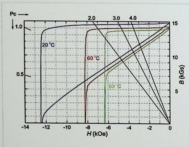
•N45 Demagnetization Curve ( II - ⑦ )
