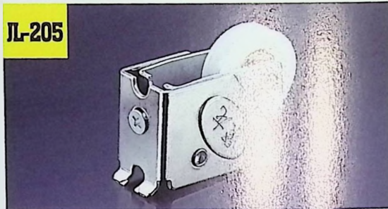
名称: 聚龙兴发2000单轮开叉 Size: 35.0X22.0X23.8mm
