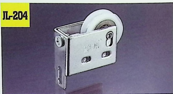
名称: 聚龙美源866单轮 Size: 28.2X17.0X18.6mm
