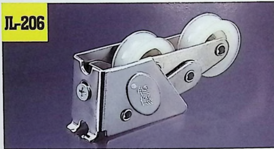
名称: 聚龙兴发2000双轮开叉 Size: 35.0X22.0X23.8mm
