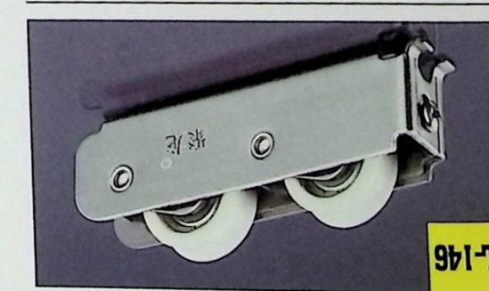
名称:聚龙97双轮 Size:26.5X18.5mm
