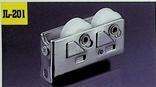
名称: 聚龙凤铝888双轮 Size: 30.0X17.2X20.0mm
