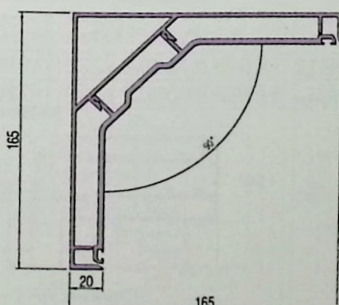
转角扣盖•Y140-105 \delta=2.5 3.292 \text{kg/m} 转角压板•Y140-106 \delta=3.5 2.647 \text{kg/m}
