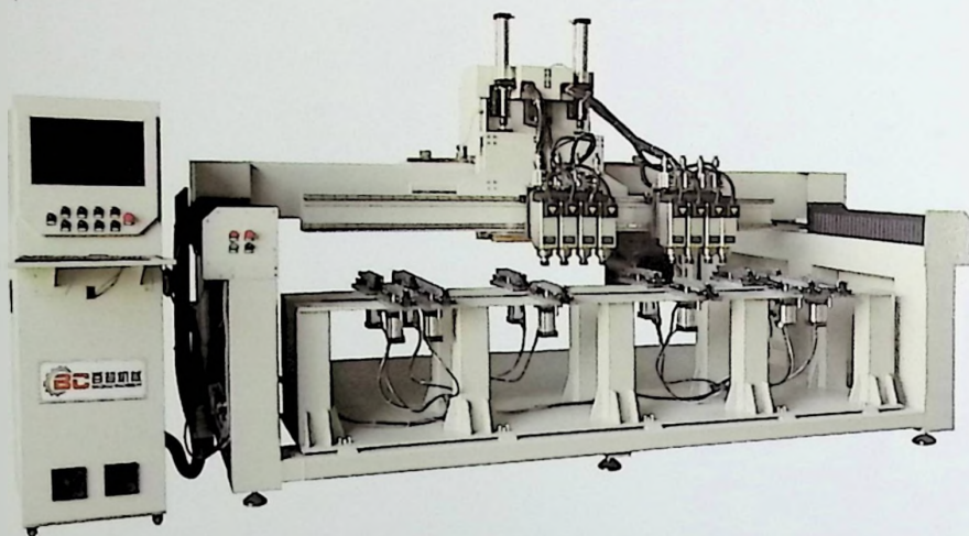
LZZ4 铝幕墙多头组合钻床 Multi-head Combination Drilling Machine
