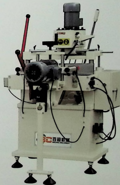
LZF3-300×100 铝型材锁孔槽加工机 Lock Hole Processing Machine
