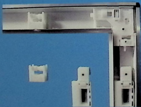
型材拼接 profile connection
