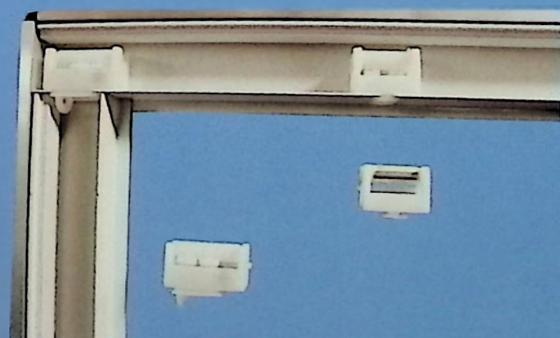
型材拼接1 profile connection 1
