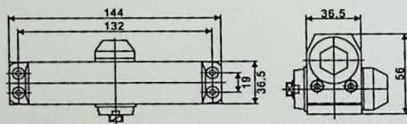
CY-061AE 圆型闭门器(B3) Round door closer (B3)
