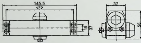
CY-051CF 方型闭门器(B2) Hexagonal door closer (B2)
