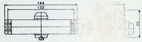
CY-061AE 方型闭门器(B3) Hexagonal door closer (B3)
