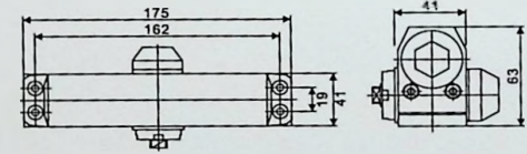
CY-061BF 方型闭门器(B3) Hexagonal door closer (B3)
