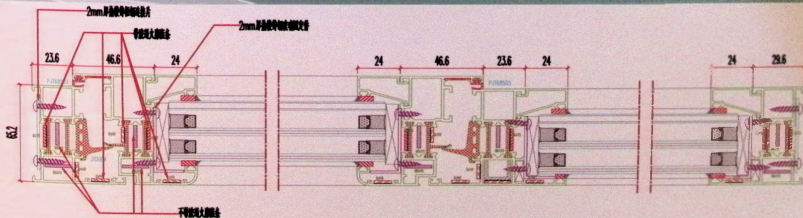
膨胀固化胶条 (30倍膨胀) Expansion curing strip
